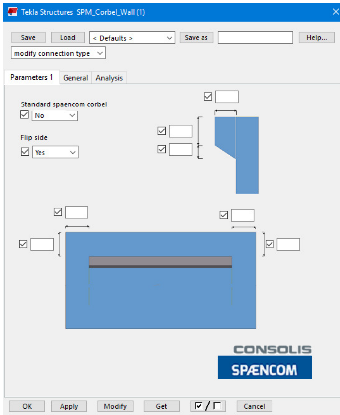
SPM_Corbel_Wall
